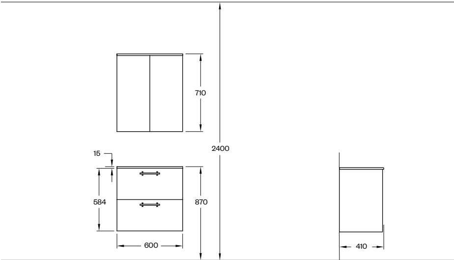
H3/60S H3/60S WARM GREY H3/MC—60 WARM GREY PORCELAIN
