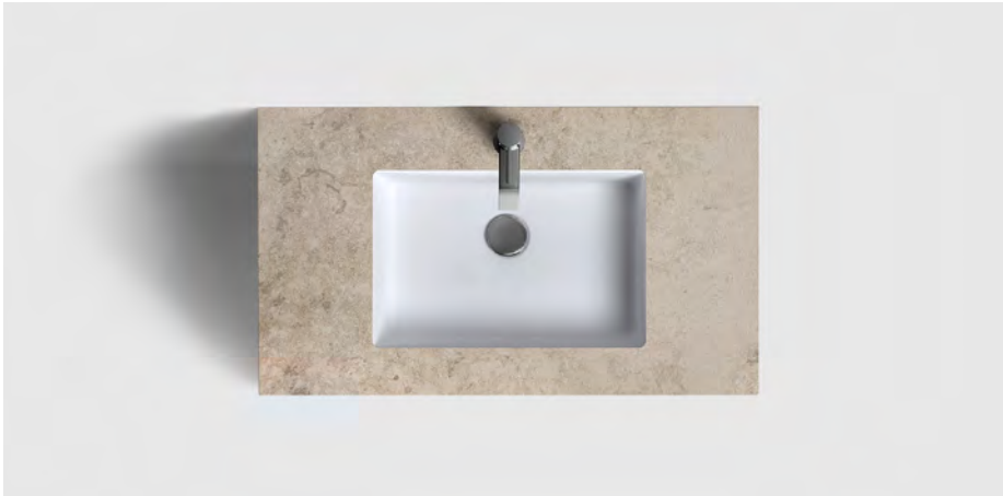
UM/80 PORCELAIN/SOLID SURFACE 465x810x12 MM/UNDERMOUNTED SINK 420x270 MM
